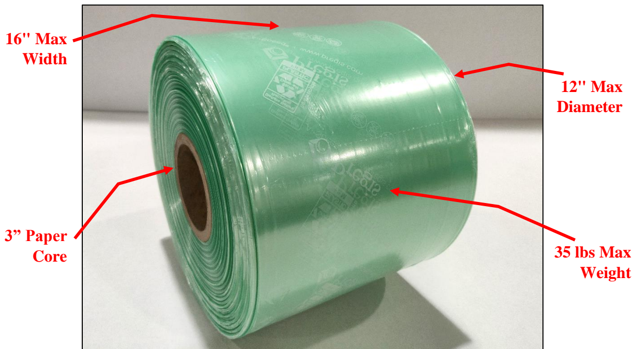
Figure 2. Supported roll dimensions.
