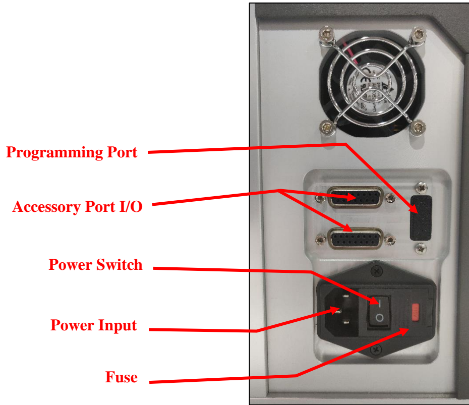
Figure 3. Inputs and Outputs.
