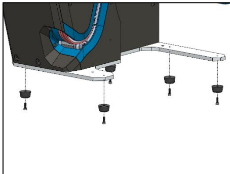
Figure 4. To remove or fasten the five rubber feet, use a 3mm hex wrench. (All five shown.)
