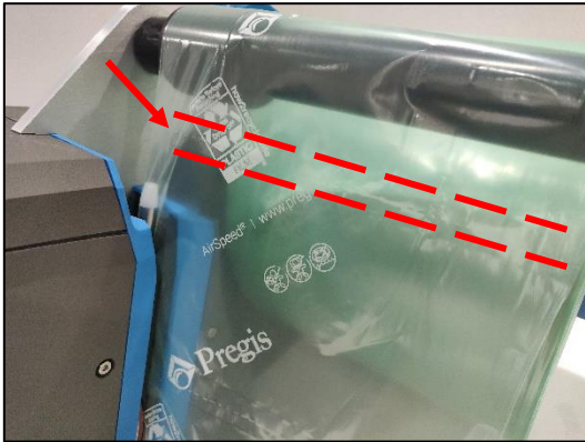
Figure 12. Tear the film along a perforation between the roller and the air channel.
