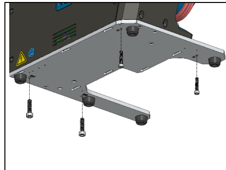
Figure 5. To mount the machine to a stand or frame, use a 6mm and 5mm hex wrench.
