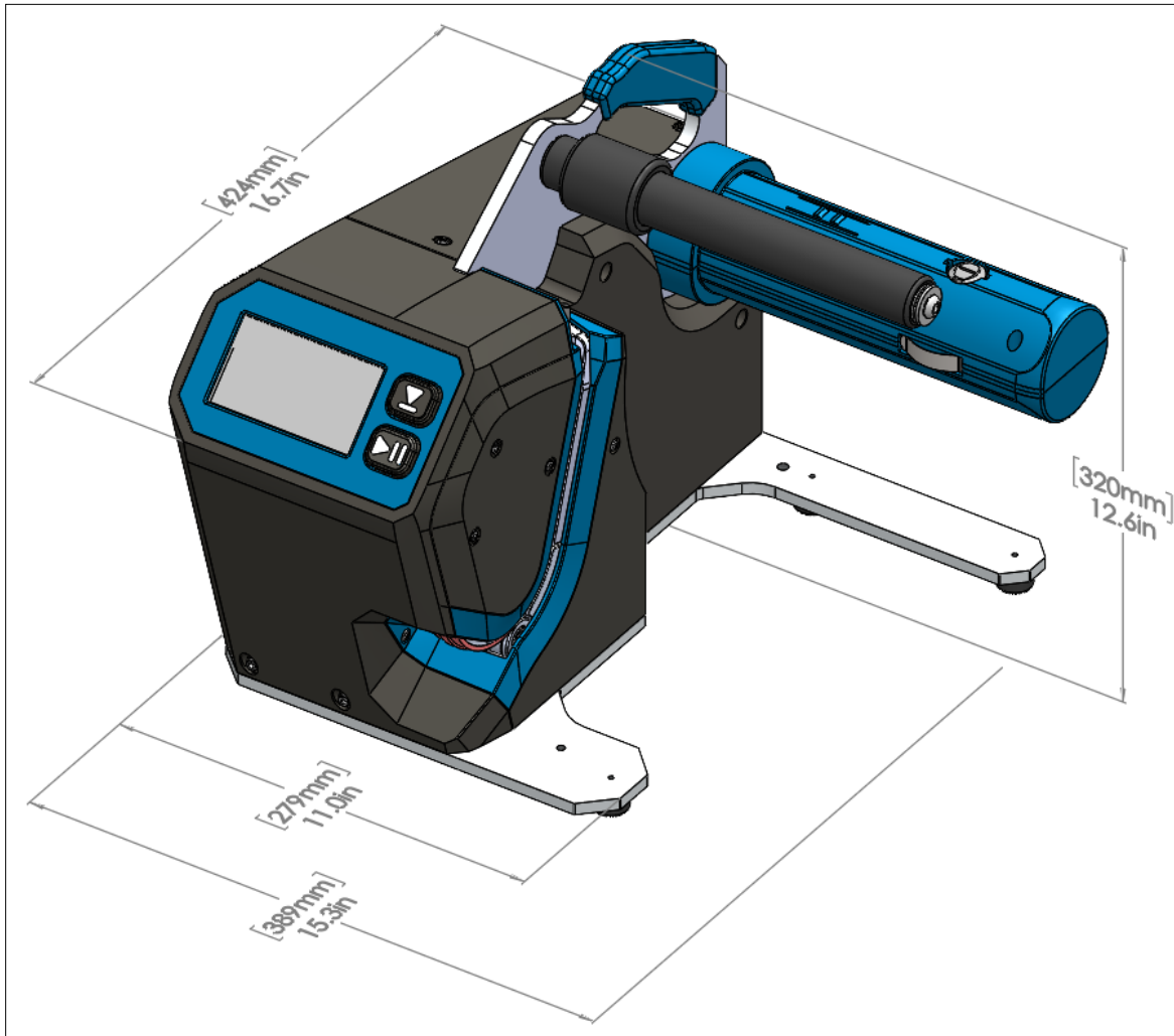
Figure 1. Machine dimensions.
