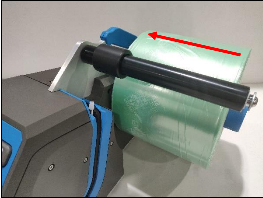
Figure 6. With the air channel first, slide the film roll onto the Spindle.
