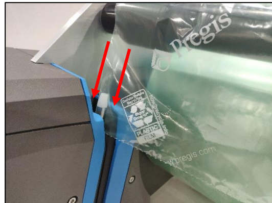
Figure 9. Thread the Air Tube into the air channel.
