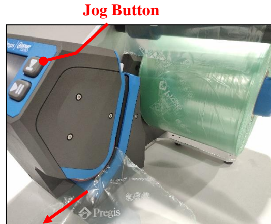
Figure 13. Use the Jog button to pass the remainder of the film through the machine.
