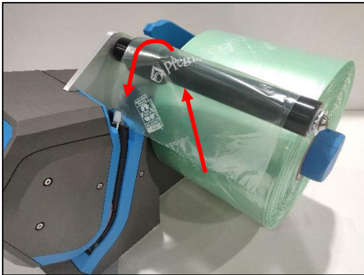
Figure 8. Pull the film off the roll and over the Guide Roller.
