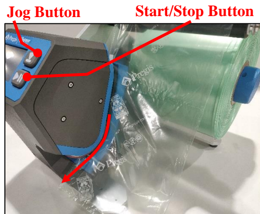
Figure 11. While holding down the Jog button, pull the film past the Nip Roller (lower, black wheel).
